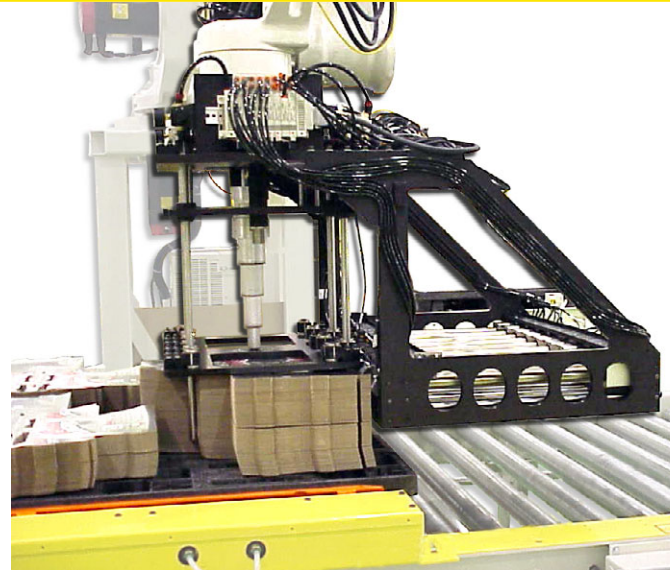
FANUC M-410i robot handling stacks of folding cartons.
